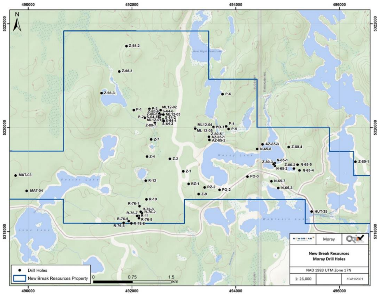
Figure 10.1: Historical Moray Gold Property Drillhole Collar Locations GIS Referenced from Various Assessment Files
