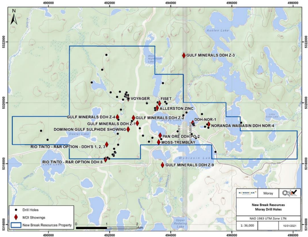
Figure 18.1: Moray Gold Property with OMDI Showings
